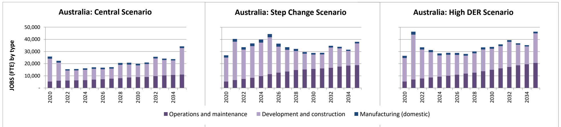
Figure 5 Share of operation and maintenance jobs, all technologies, 2020-2035
