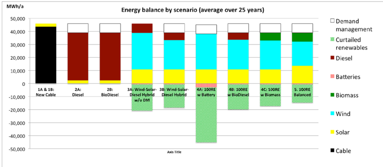
Figure 7: Scenarios Energy production (MWh/year)
